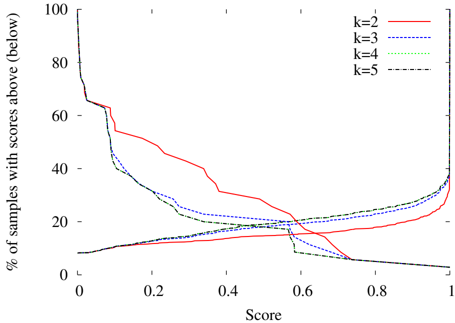
Fig. 7: Malware and Goodware Recognition. Timeouts for generating the dependency graphs were 120sec for malware test and training sets and 800sec for the goodware test set in the figure on the left. The training set consists of 50% of the entire malware set, chosen at random. The test set consists of the remaining malware samples (curves rising from left to right), and the goodware set (curves falling from left to right). The rising curves represent the percentage of malware samples for which the computed score was less than the corresponding value on the x axis. The falling curves represent the percentage of goodware samples for which the score was greater than the corresponding value on the x axis. The figure shows curves for four different values of k , there is essentially no difference between the cases when k = 4 and k = 5 . For the rising curves, the lowest curve is for k = 2 , the next higher one for k = 3 , and the two highest ones for the remaining cases. For the falling curves, the ordering is reversed. The optimal score for distinguishing malware from goodware is the lowest intersection of the rising and falling curves for the same k .
